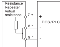
3-wire (+, -, -)
